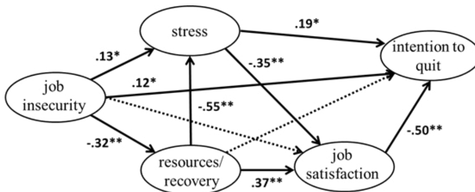
Figure 2. Structural equation modeling (SEM)–joint sample
