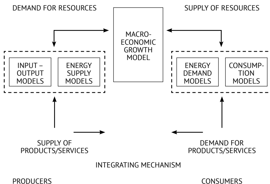
Figure 1. Energy-economy model
